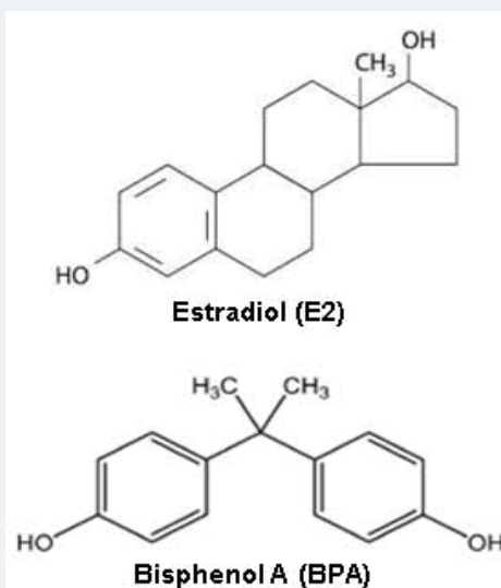
Figure 1: The structures of endogenous estrogens and BPA.
