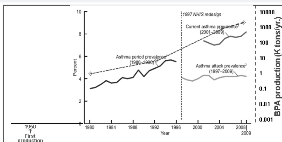
Figure 2: Temporal relationships between the increases of asthma prevalence and BPA production.
